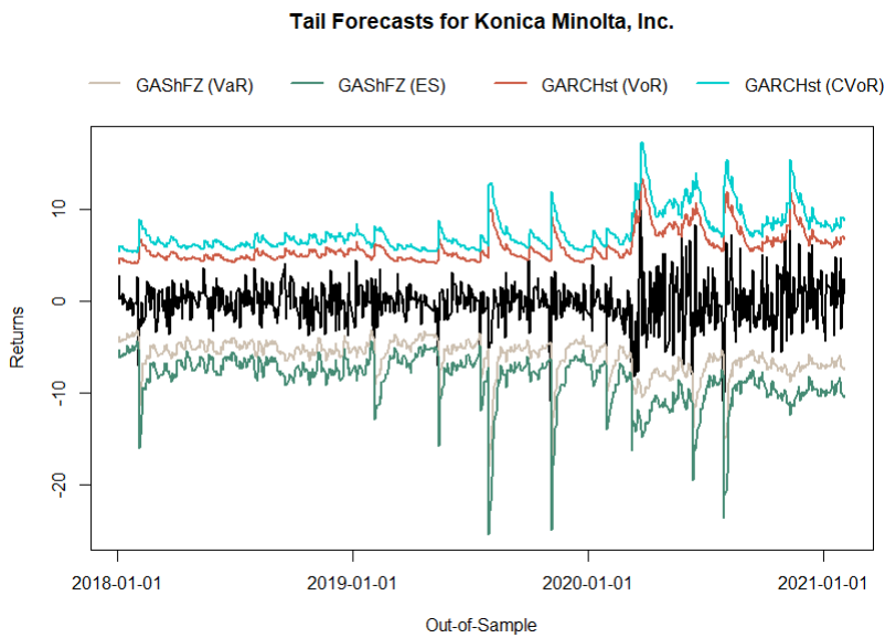
Figure S19 Example top ESG Japan (ESG = 81.5, ESGR = 13.5) forecasted tail measures.
