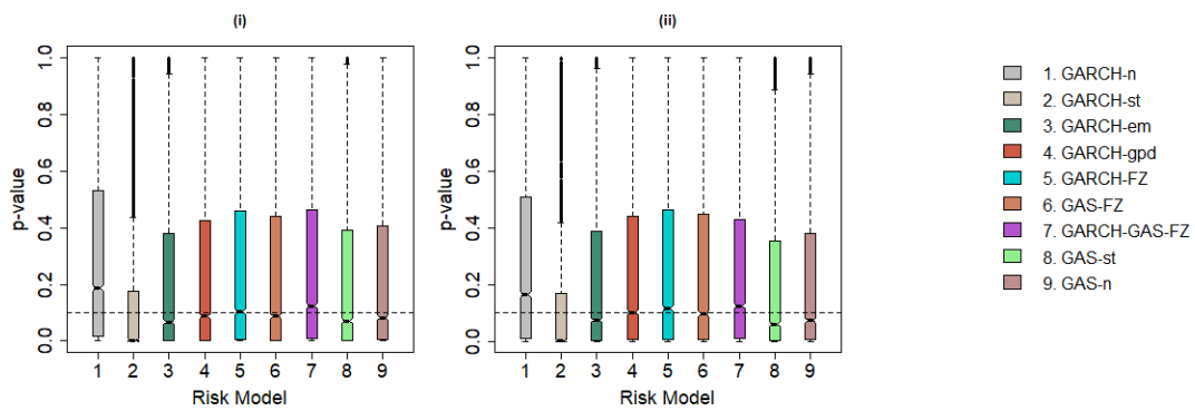
Figure S3 Goodness-of-fit for (i) VoR and (ii) CVoR at 1%.
