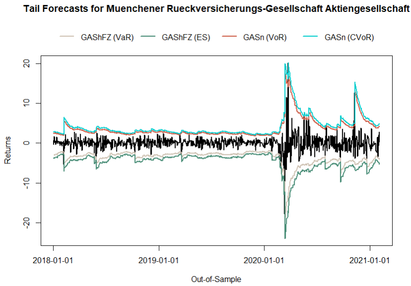
Figure S18 Example top ESG Germany (ESG = 84.7, ESGR = 16.1) forecasted tail measures.
