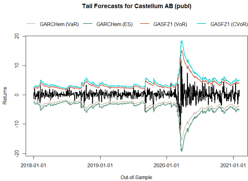
Figure S21 Example top ESG Sweden (ESG = 85.2, ESGR = 13.5) forecasted tail measures.
